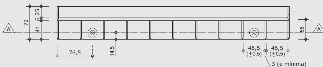
VISTA FRONTAL
