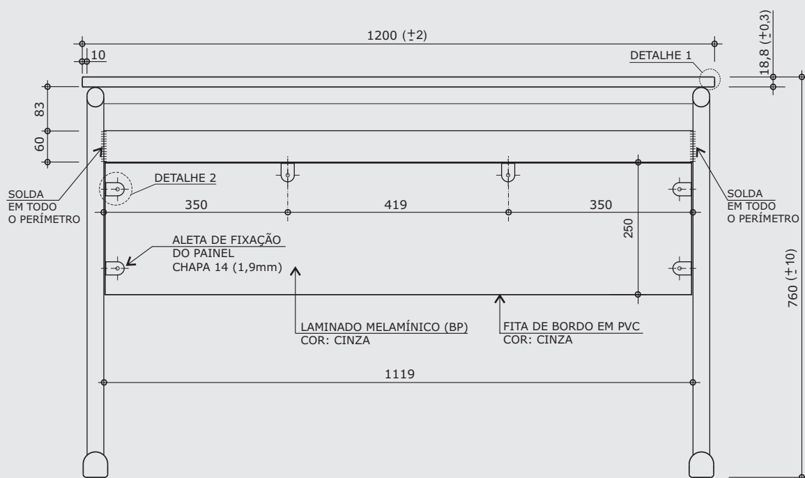
VISTA FRONTAL
