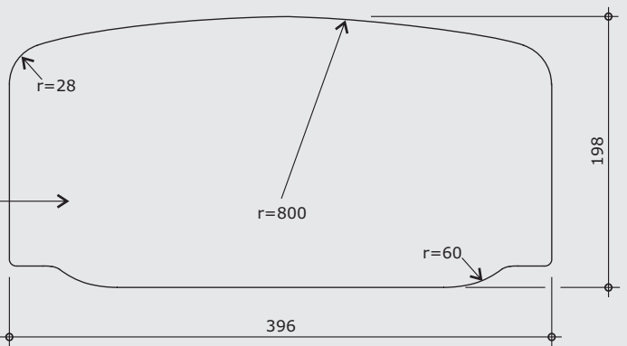
VISTA FRONTAL
